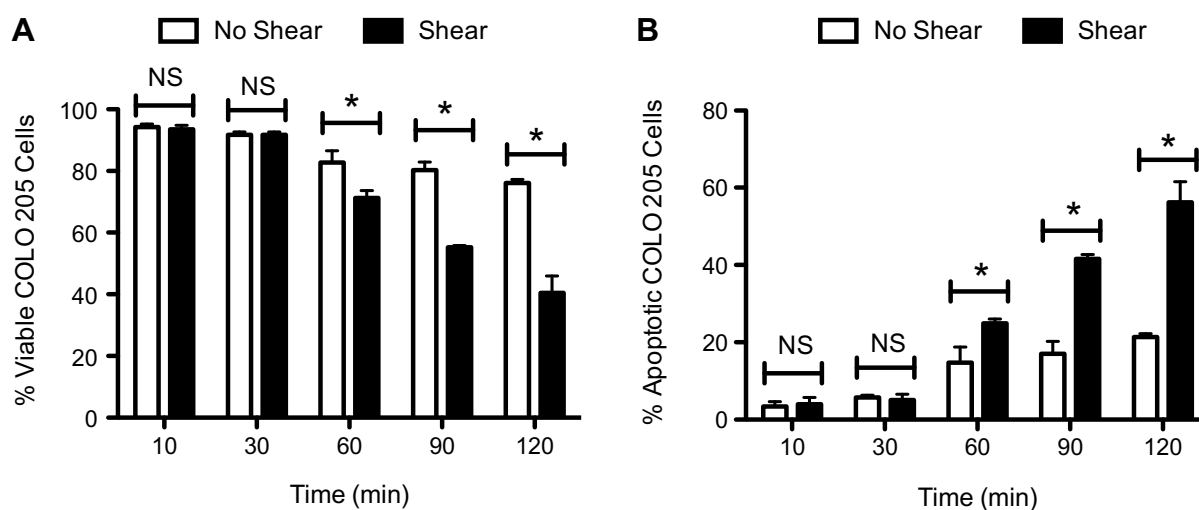
Figure 5. Shear-induced sensitization to TRAIL increases with increasing exposure time to fluid shear stress. Per cent viable (A) and apoptotic (B) COLO 205 cells ( n = 3 ). Time dependence of shear-induced sensitization was determined by increasing the fluid shear stress exposure time from 10 to 120 min at a uniform shear stress of 2.0 \text{ dyn cm}^{-2} at 37^\circ\text{C} . COLO 205 cells were treated with 0.1 \mu\text{g ml}^{-1} TRAIL prior to the onset of fluid shear stress. Error bars represent 95% confidence intervals. *P < 0.05 for all measurements.
