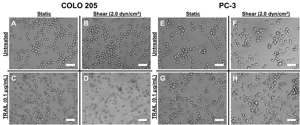
Figure 2. Brightfield microscopy images of untreated COLO 205 cells exposed to static conditions (A) and 2.0 \text{ dyn cm}^{-2} of fluid shear stress (B) for 120 min at 37^\circ\text{C} . COLO 205 cells treated with 0.1 \mu\text{g ml}^{-1} TRAIL and then exposed to static conditions (C) and 2.0 \text{ dyn cm}^{-2} of fluid shear stress (D) for 120 min at 37^\circ\text{C} . Untreated PC-3 cells exposed to static conditions (E) and 2.0 \text{ dyn cm}^{-2} of fluid shear stress (F) for 120 min at 37^\circ\text{C} . PC-3 cells treated with 0.1 \mu\text{g ml}^{-1} TRAIL and then exposed to static conditions (G) and 2.0 \text{ dyn cm}^{-2} of fluid shear stress (H) for 120 min at 37^\circ\text{C} . Scale bars = 30 \mu\text{m} .
