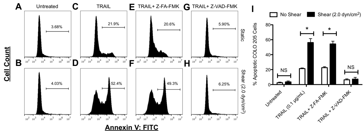
Figure 8. Fluid shear stress sensitization to TRAIL-mediated apoptosis is caspase-dependent. COLO 205 cells (A, B) treated with 0.1 \mu\text{g ml}^{-1} TRAIL (C, D), negative control inhibitor Z-FA-FMK followed by 0.1 \mu\text{g ml}^{-1} TRAIL (E, F), and pan caspase inhibitor Z-VAD-FMK followed by 0.1 \mu\text{g ml}^{-1} TRAIL (G, H), exposed to static conditions and 2.0 \text{ dyn cm}^{-2} of fluid shear stress for 120 min at 37^\circ\text{C} , respectively. Per cent apoptotic COLO 205 cells ( n = 3 ) after exposure to various treatments (I). Gated region of flow cytometry histograms represents apoptotic COLO 205 cells. Gates determined by labeling viable COLO 205 control samples with Annexin-V FITC staining. FITC: fluorescein isothiocyanate. NS: non-significant.
