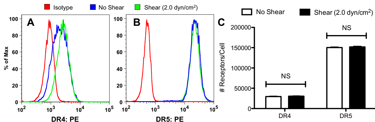
Figure 9. Fluid shear stress does not alter death receptor surface expression. COLO 205 cells exposed to static conditions and 2.0 \text{ dyn cm}^{-2} of fluid shear stress for 120 min at 37^\circ \text{C} were labeled with anti-DR4 (A) and anti-DR5 (B) antibodies, respectively. (C) QSC receptor quantification of DR4 and DR5 on the surface of COLO 205 cells exposed to static conditions and fluid shear stress ( n = 3 ). NS: non-significant.
