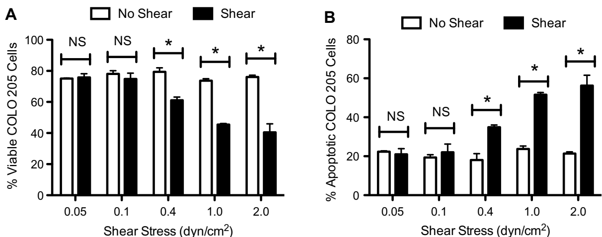
Figure 4. Increasing fluid shear stress sensitizes cancer cells to TRAIL. Per cent viable (A) and apoptotic (B) COLO 205 cells ( n = 3 ). Shear stress magnitude was varied in separate experiments from 0.05 to 2.0 \text{ dyn cm}^{-2} for 120 min at 37^\circ\text{C} . COLO 205 cells were treated with 0.1 \mu\text{g ml}^{-1} TRAIL prior to the onset of fluid shear stress. Error bars represent 95% confidence intervals. *P < 0.05 for all measurements.
